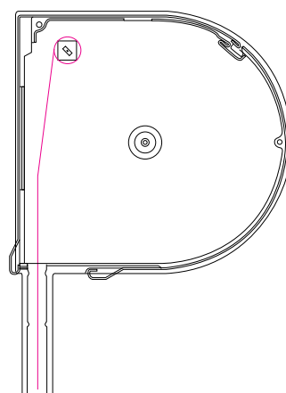
Cross-section of a half-round box with a mosquito screen
